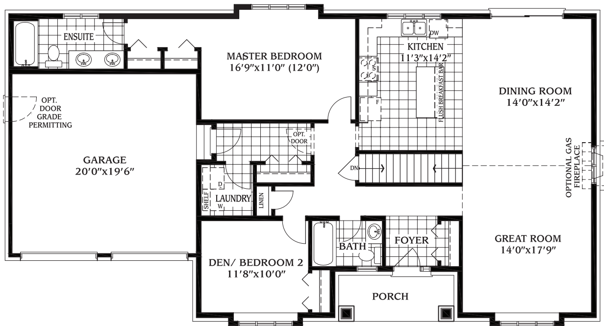
MAIN FLOOR 1,620 sq. ft.
